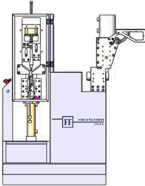
MPK-16 Looper
